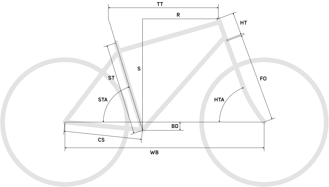
FS = ST frame size = seat tube [mm] TT top tube [mm] HT head tube [mm] HTA head tube angle [°] STA seat tube angle [°] CS chain stay length [mm] BD bottom bracketed drop [mm] FO fork length [mm] S stack [mm] R reach [mm] WB wheel base [mm]
